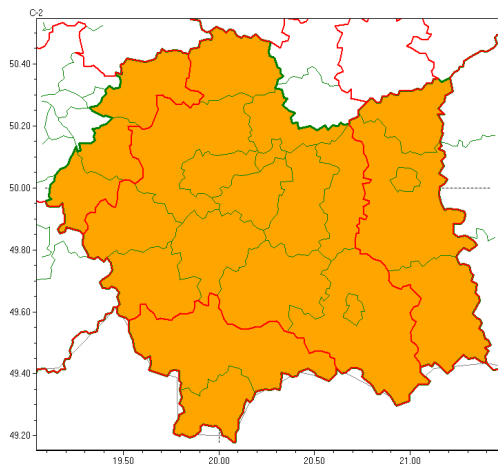
Burze z gradem 2022-06-28 14:46
